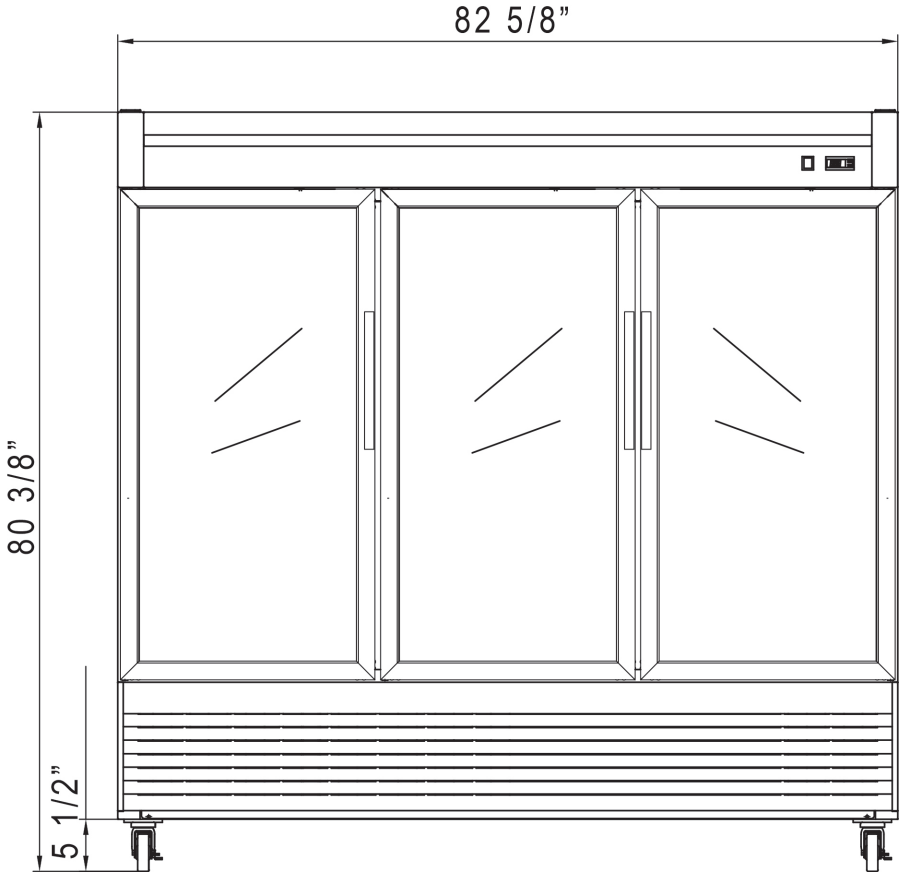
Front View
